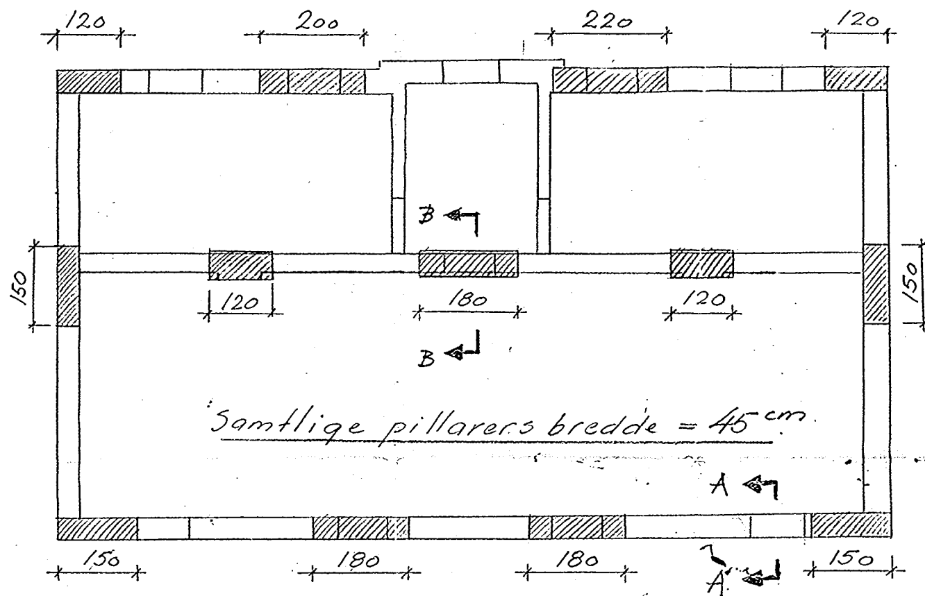
Pillarplan 1:100.
